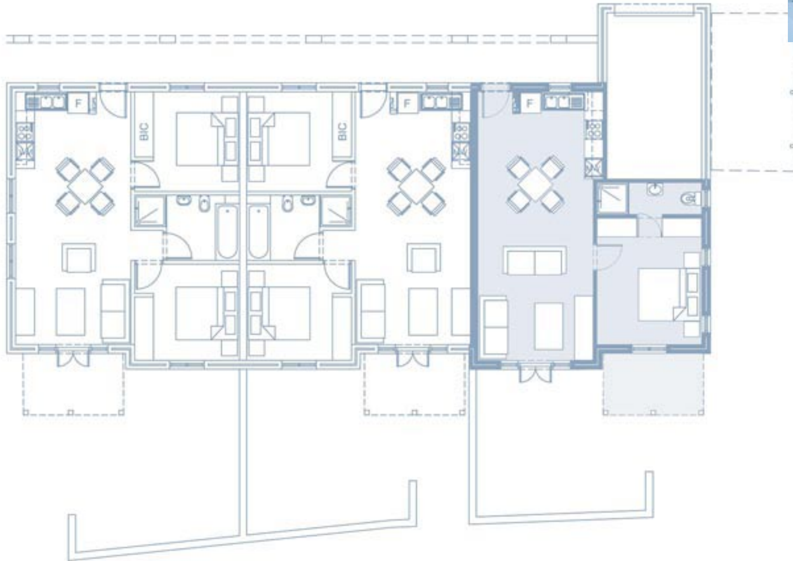
THE LAKE SIDE FLOORPLANS
