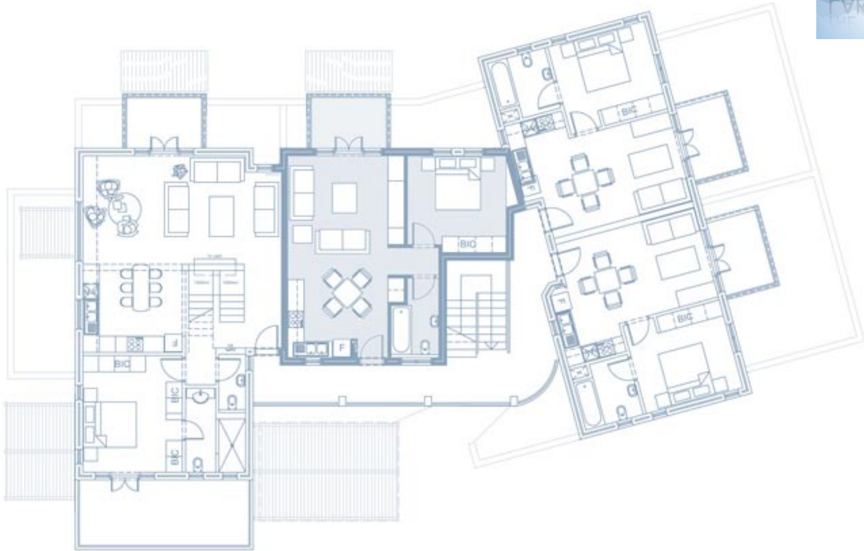
THE LAKE SIDE FLOORPLANS
